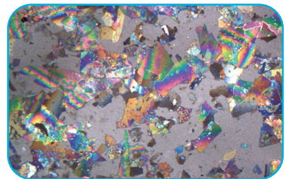
Glass delamination flakes from the interior wall of a delaminated pharmaceutical vial as seen using coaxial illumination.
